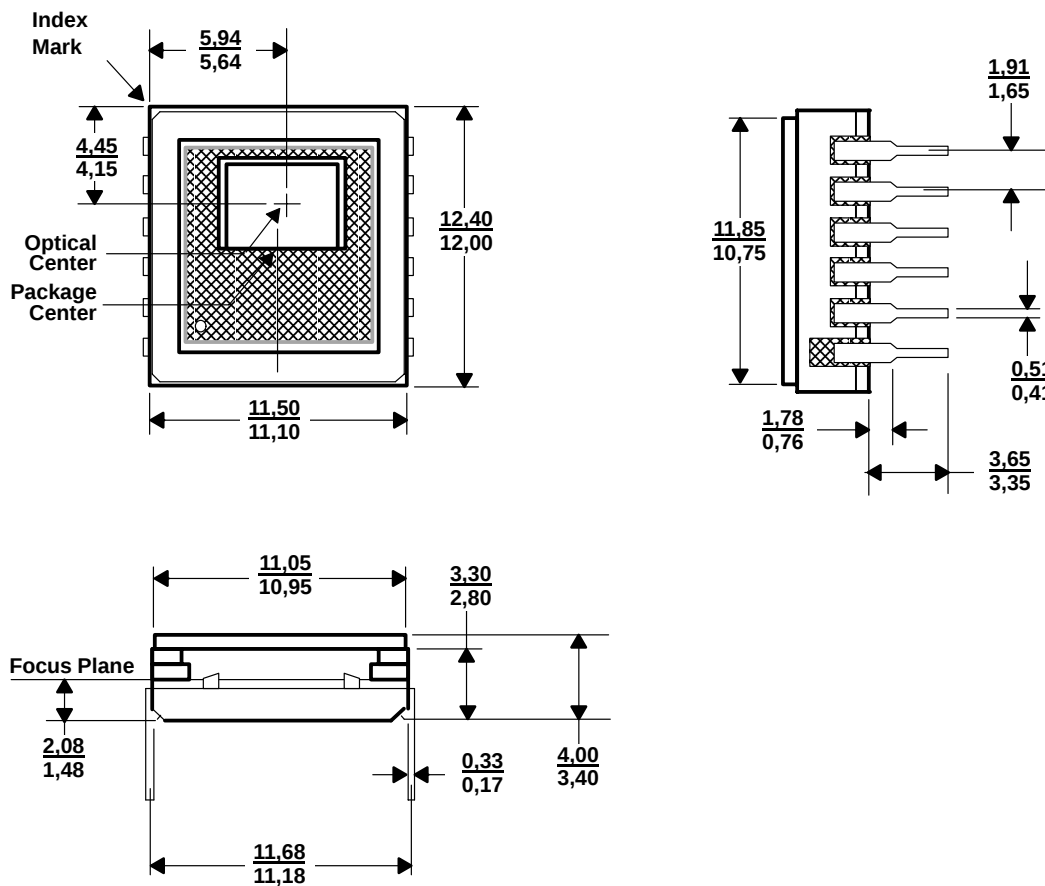
TC237 (12 pin)
